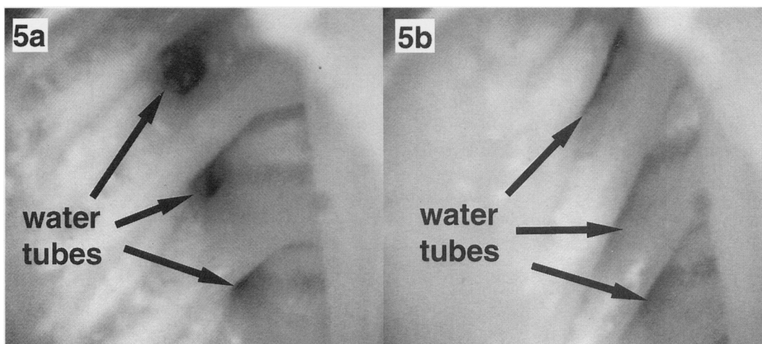
Figure 5. Endoscopic observations. Water tubes are seen at the position where they empty into the suprabranchial chamber of Lampsilis anodontooides . During active pumping, the tubes are open (a); when the muscles of the gill and gill axis contract, the water tubes are drawn together and largely close the tubes (b). This type of contraction takes about 1–5 s.
