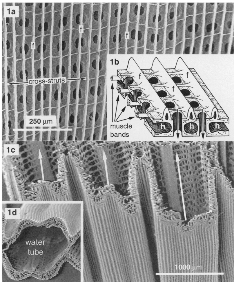
Figure 1. Eulamellibranch gill organization and water flow. (a, b) General organization of a single gill lamella with epithelial tissue removed to reveal the organization of the supporting structures (modified from Medler and Silverman, 1998, with permission from Invertebrate Biology ). (a) Dreissena polymorpha gill (SEM) showing parallel filaments ( f ) held apart by connective tissue cross-struts. Bands of smooth muscles are found below the cross-struts (b); during muscle contraction, the cross-struts bend inwardly and the filaments are drawn closer to one another. In addition to these muscle bands, more diffuse smooth muscle fibers (depicted as thin wavy lines) are found in the connective tissue sheets that enclose the hemocoel ( h ) at the base of the filaments (b). Water is drawn into the central water channel of the gill through water canals (indicated by arrows in b). Ostia (dark openings perforating the gill lamellae) represent the ends of the water canals and provide a route for water to flow into the central region of the gill. (c, d) Frontal (c) and cross-sectional (d) views (SEM) of Mercenaria mercenaria gill, demonstrating the movement of water (indicated by arrows in c) through the water tubes of the gill after entering the gill through the water canals. The route of water flow through the gill is between the gill filaments and then through the gill ostia and associated water canals. Water moves to the suprabranchial chamber (not shown) through the water tubes of the central water channel. The suprabranchial chamber at the top of each gill is connected directly to the excurrent aperture where the water leaves the animal.
